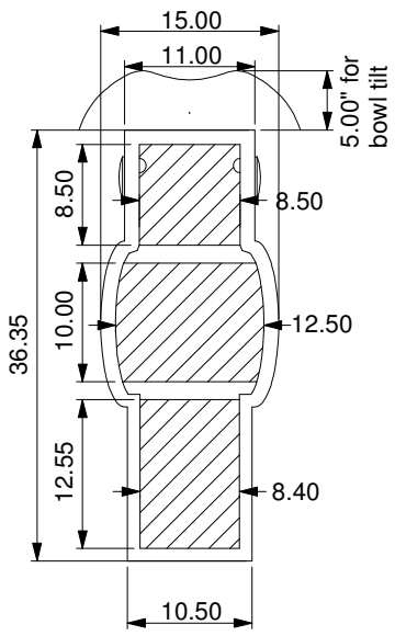
Shroud Bottom
